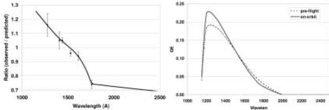
Figure 7. Left : Preliminary comparison between observed and predicted count rates using the pre-flight response curve for the SBC. Solid line shows the derived correction. Right : Pre-flight and corrected quantum efficiency for the SBC MAMA.
