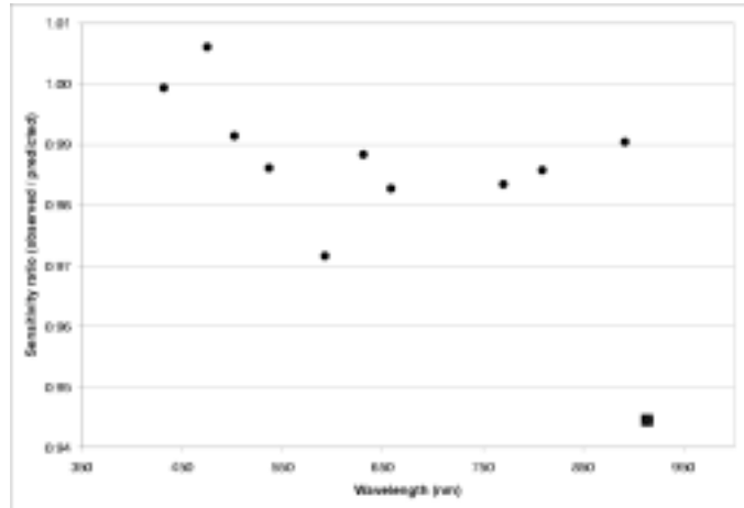
Figure 4. Ratio of observed to predicted count rates using the new WFC detector QE curve
