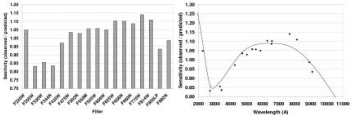
Figure 5. Left : ratio of observed-to-predicted count rates using the pre-flight estimates of the response curves for HRC. Right : Circle show the average ratio for the two standard stars observed in June and July. The solid line shows the derived correction curve for the response.
